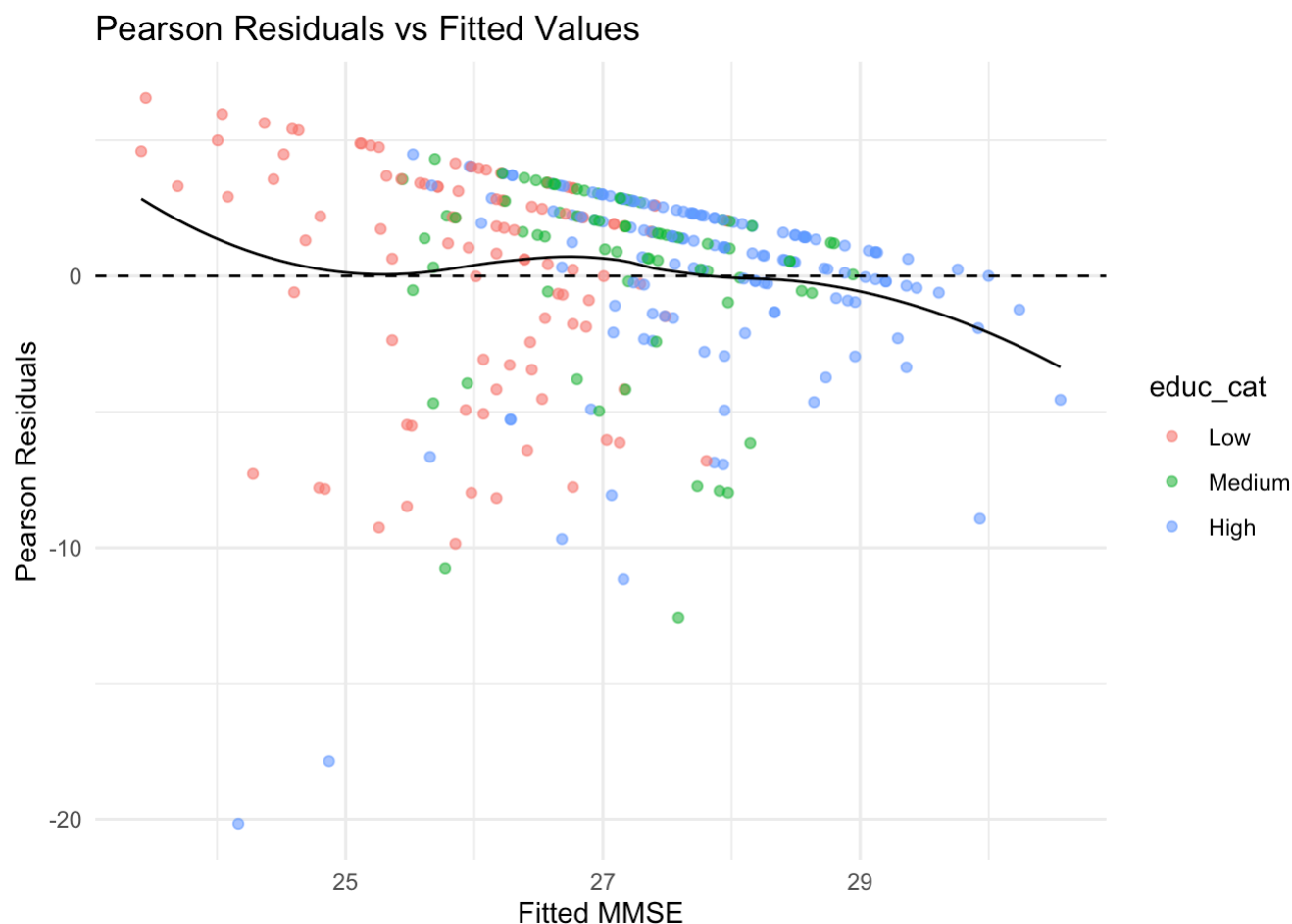
Figure 11: Pearson Residuals vs Fitted Values
