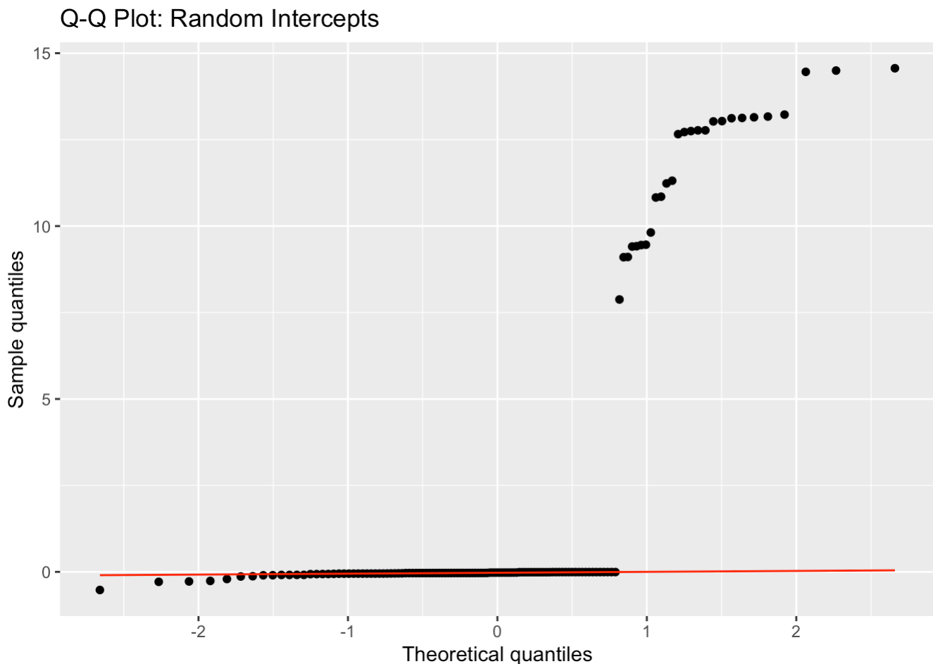
Figure 15: Q-Q plot
